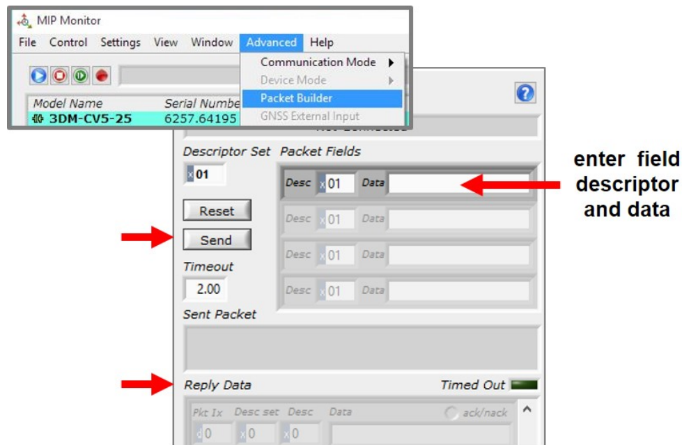
Figure 35 -Packet Builder
