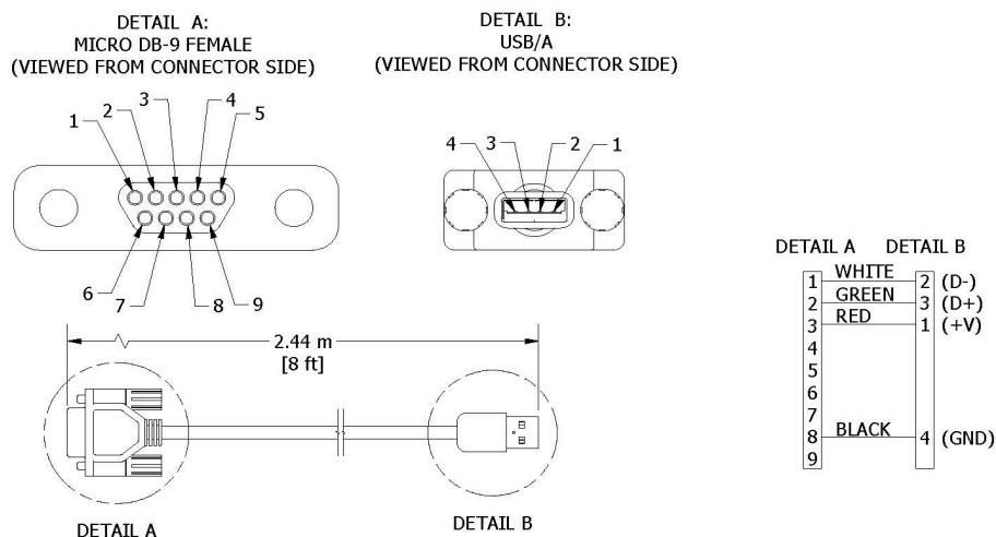
Figure 43 - USB Communications cable
