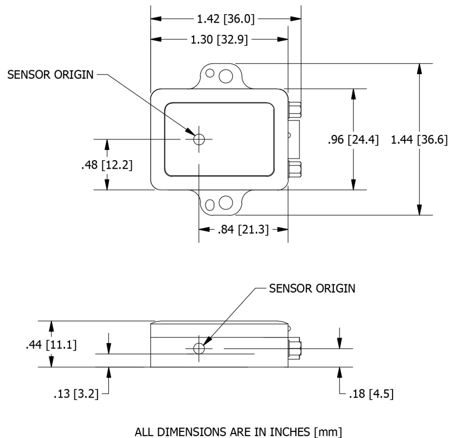
Figure 41 - 3DM-GX5-25 Sensor Origin
