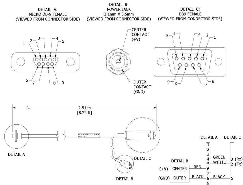
Figure 42 - RS232 Communications and power cable
