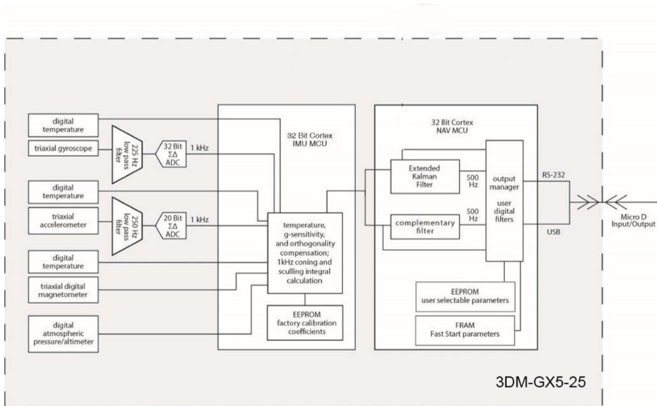
Figure 15 - 3DM-GX5-25 Block Diagram
