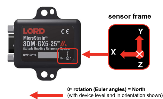
Figure 20 - Sensor Frame
