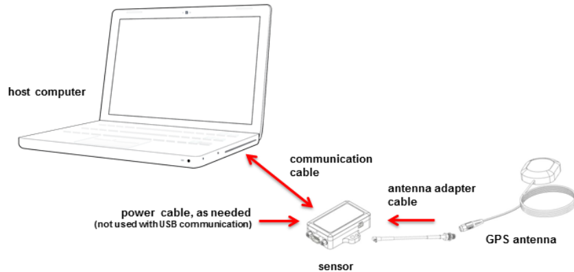
Figure 4 - System Connections
