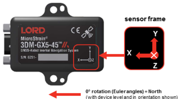
Figure 19 - Sensor Frame
