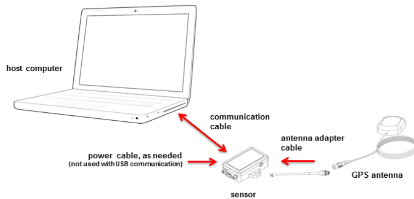
Figure 5 - System Connections
