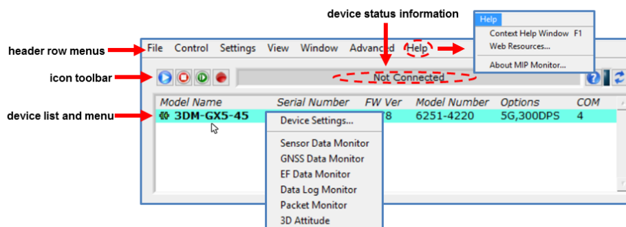
Figure 6 - Main Window
