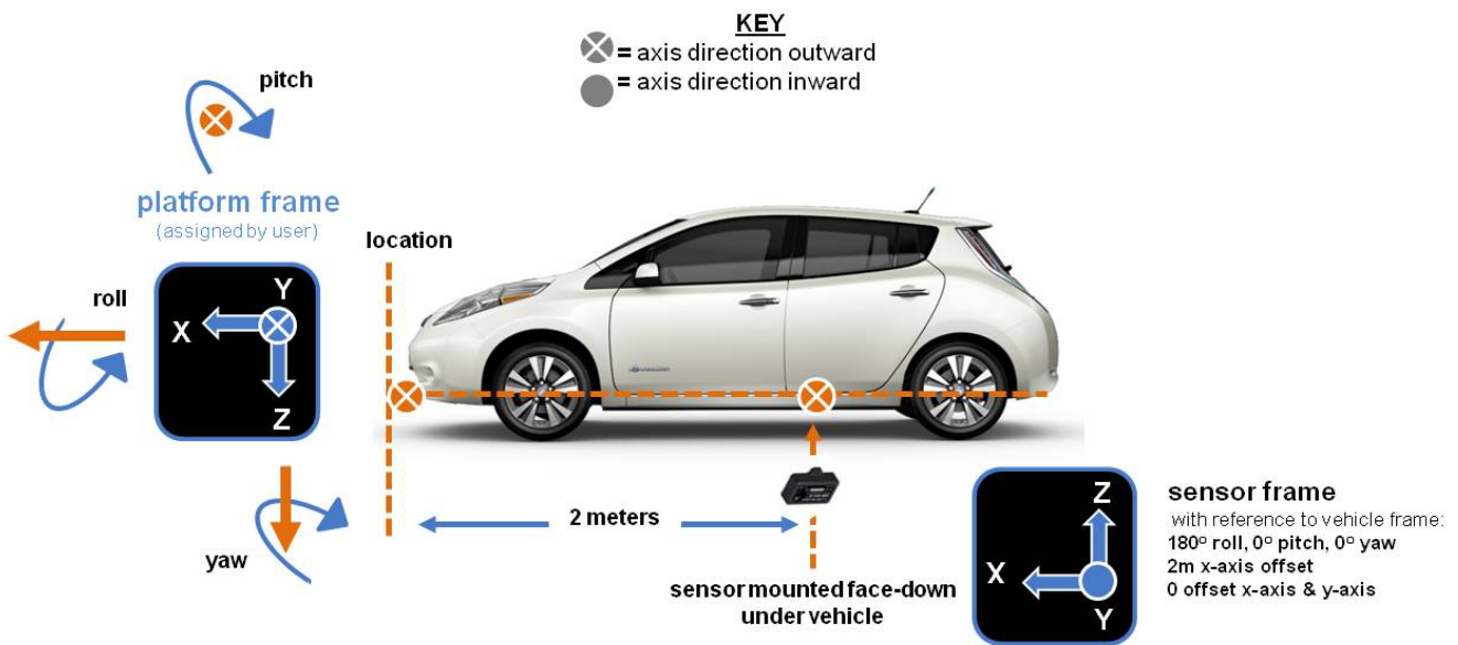
Figure 20 - Platform Frame Transformation
