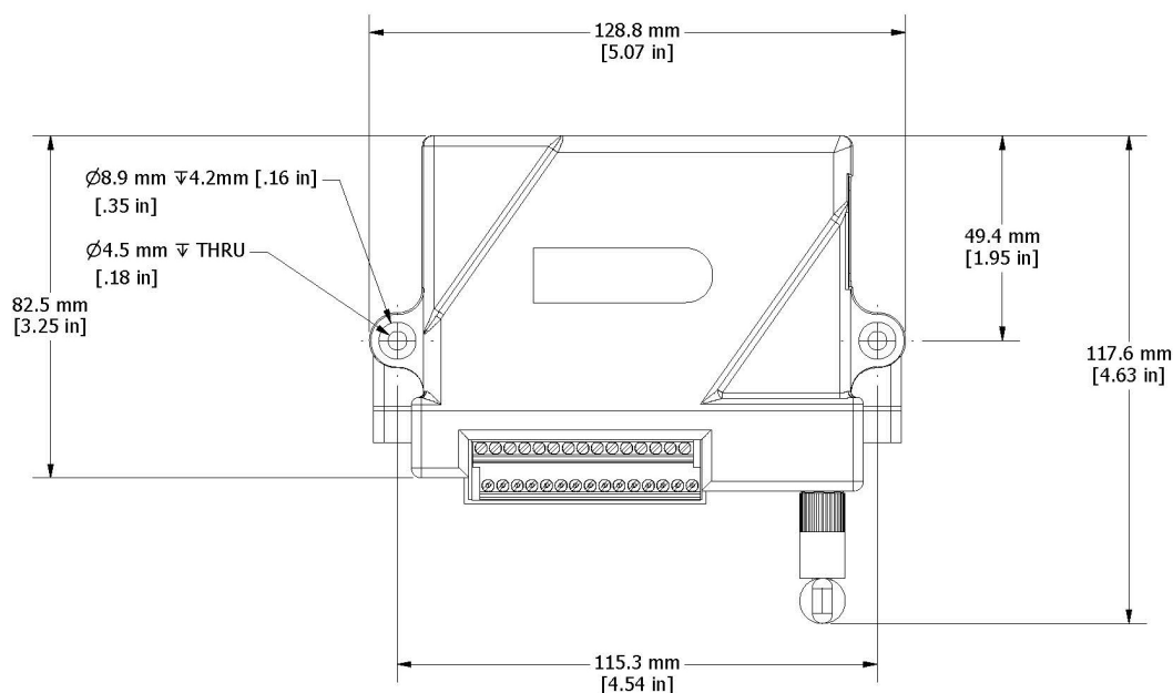
Figure 25 - Mounting the Node
