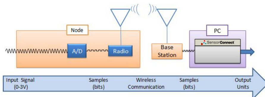
Figure 32 - Single Ended Signal Processing
