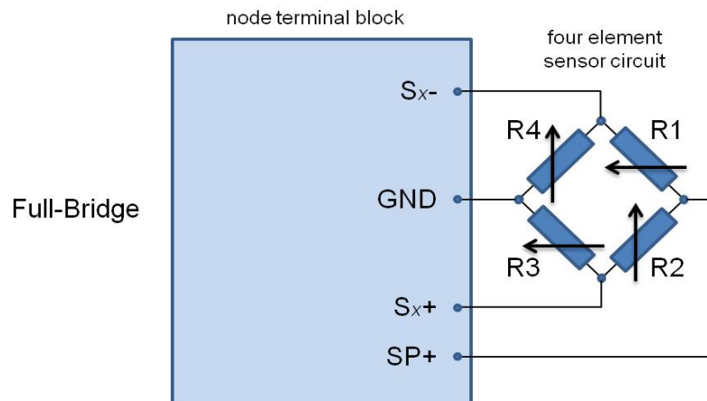
Figure 29 - Full Bridge Wiring
