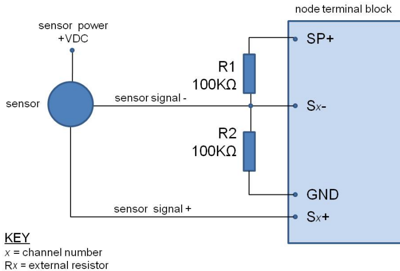
Figure 31 - Small Voltage Measurement
