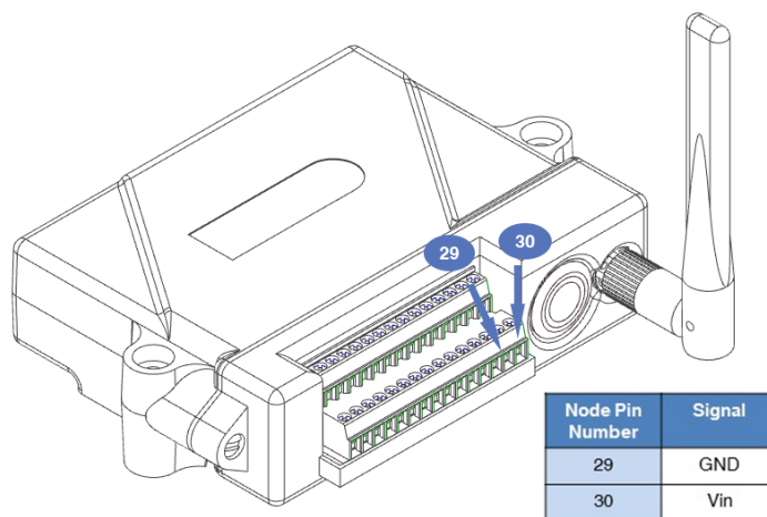
Figure 49 - External Power Connection
