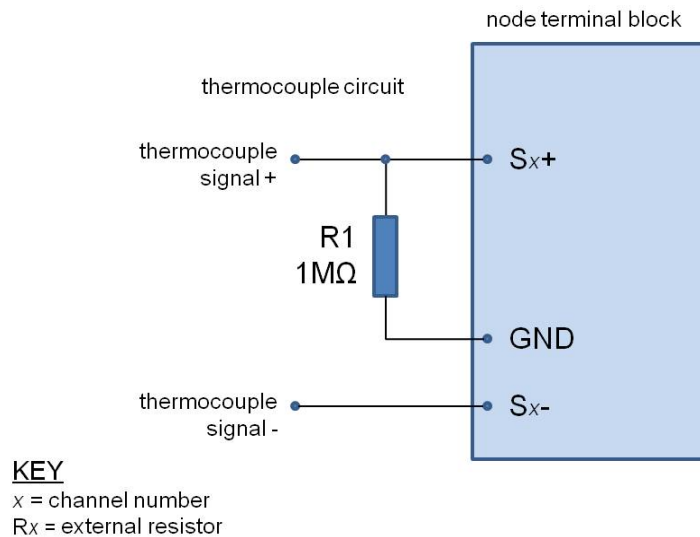
Figure 34 - Connecting a Thermocouple
