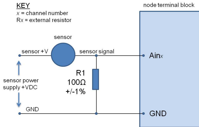
Figure 33 - Small Current Measurements
