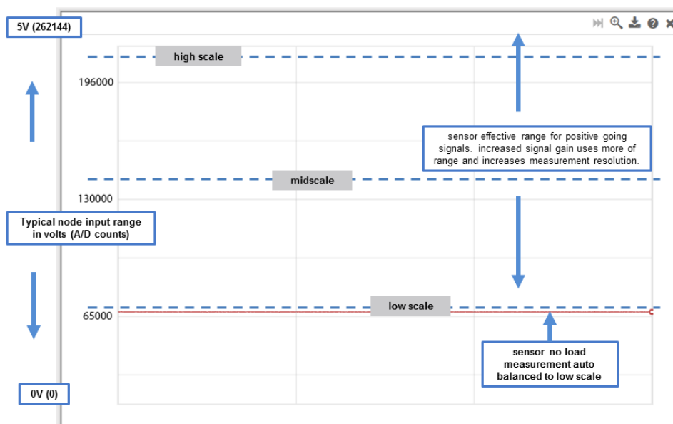
Figure 48 - Differential Input Resolution and Offset (18-bit Node)
