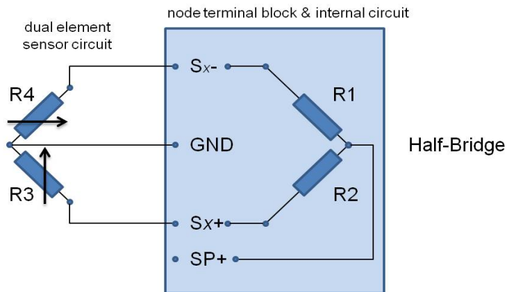
Figure 30 - Half and Quarter-Bridge Wiring
