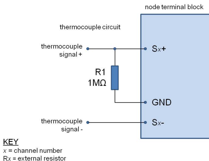
Figure 34 - Connecting a Thermocouple
