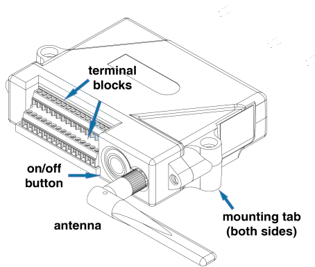
Figure 2 - Interface and Indicators
