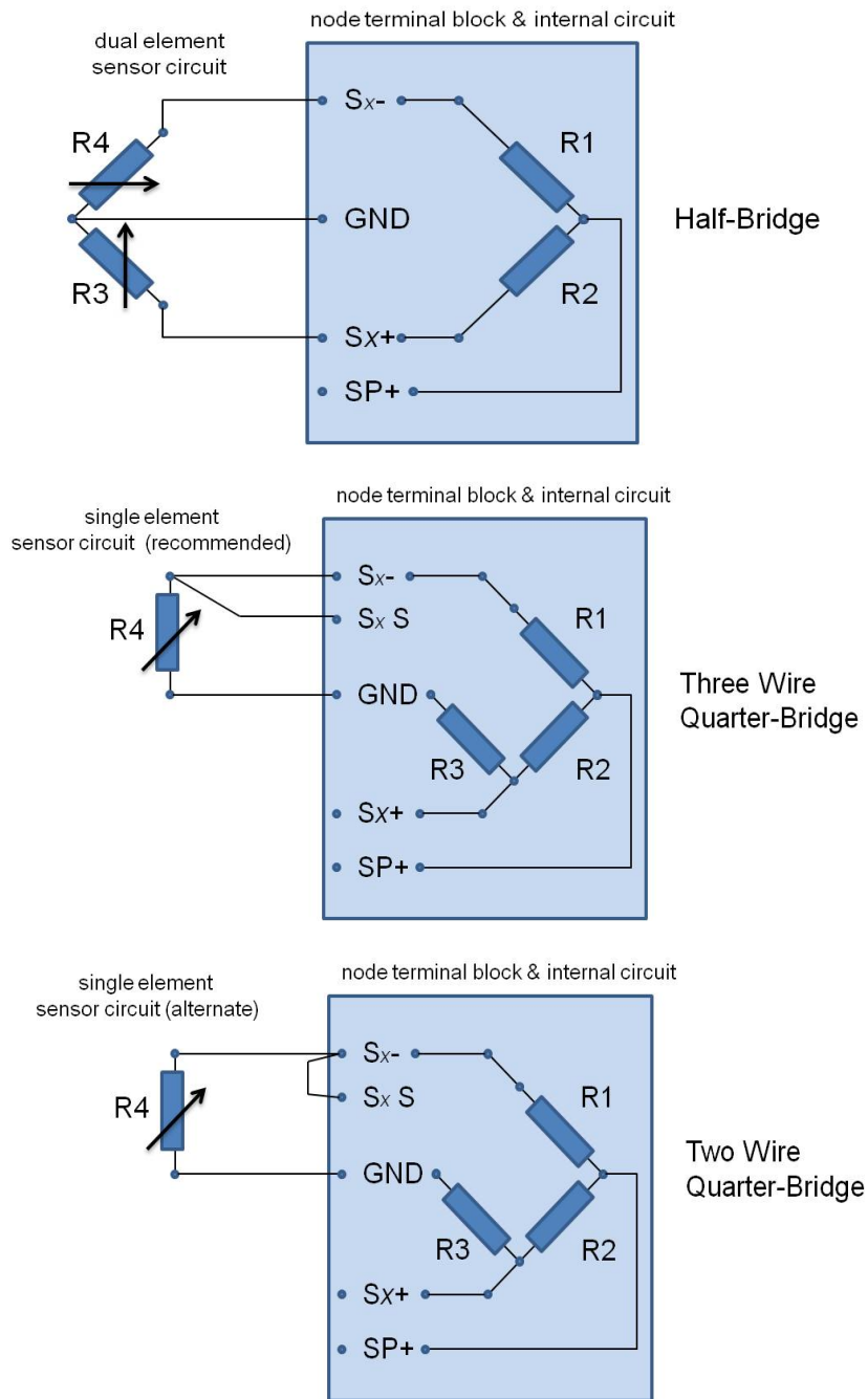
Figure 30 - Half and Quarter-Bridge Wiring
