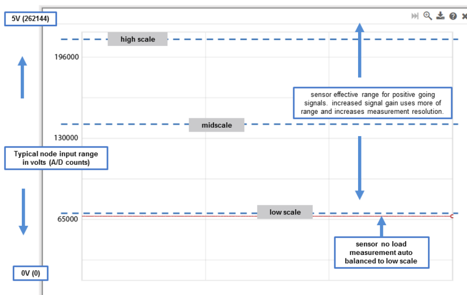
Figure 48 - Differential Input Resolution and Offset (18-bit Node)
