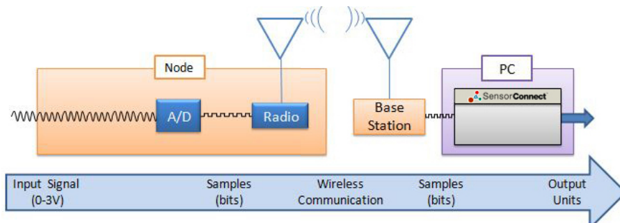
Figure 32 - Single Ended Signal Processing
