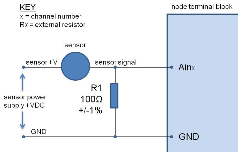
Figure 34 - Small Current Measurements
