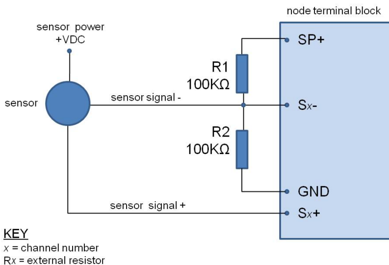
Figure 32 - Small Voltage Measurement
