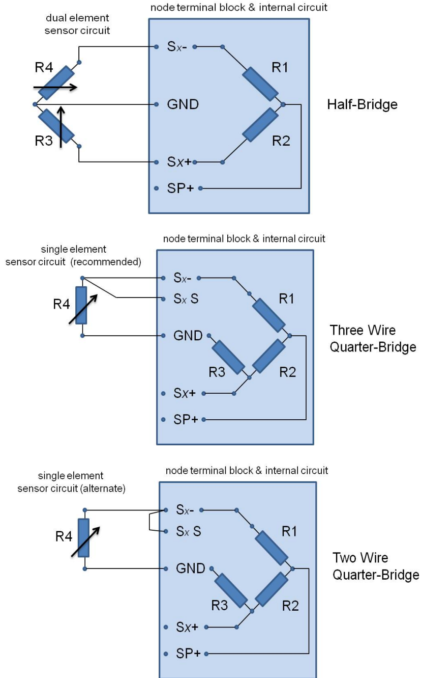
Figure 31 - Half and Quarter-Bridge Wiring
