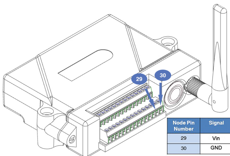
Figure 50 - External Power Connection
