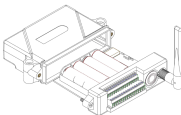
Figure 57 - Replace Batteries
