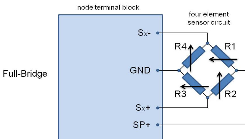
Figure 30 - Full Bridge Wiring
