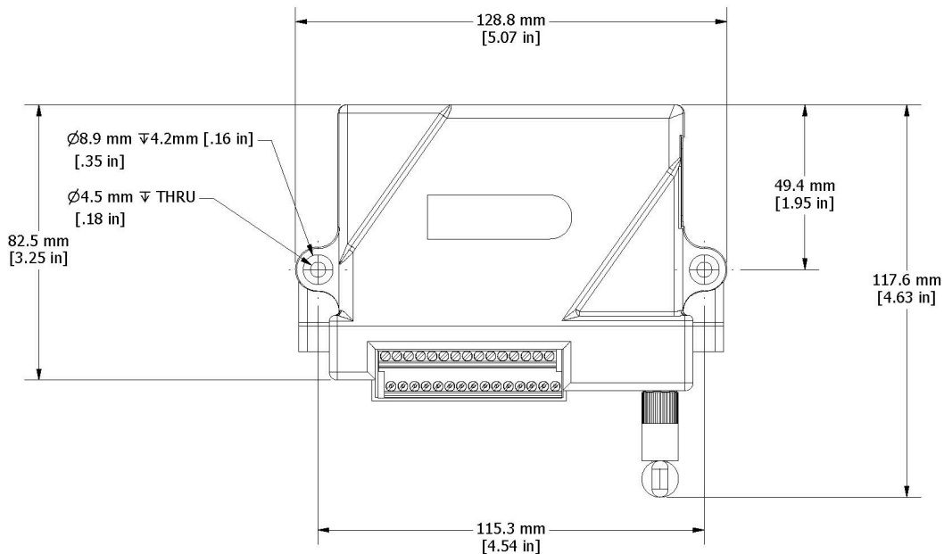
Figure 26 - Mounting the Node
