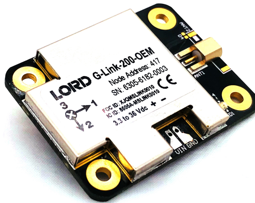
Figure 1 - G-Link-200-OEM
