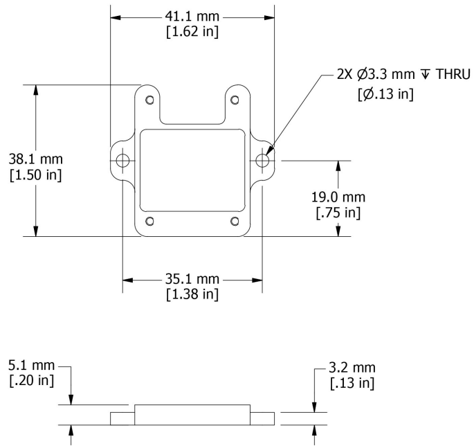
Figure 35 - Installing the Mounting Board
