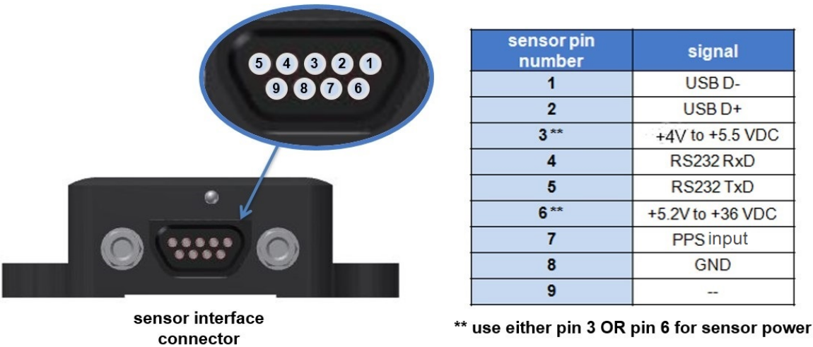
Figure 37 -Connector Wiring
