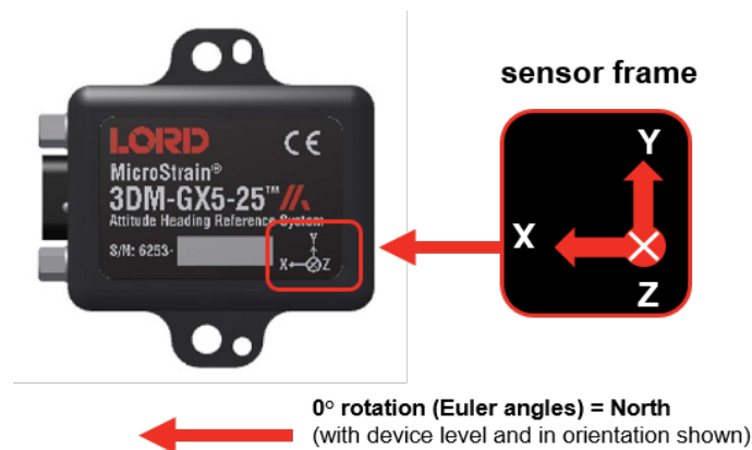
Figure 19 -Sensor Frame
