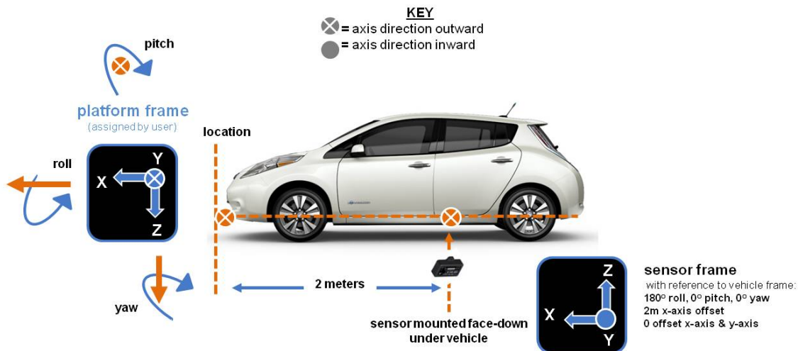
Figure 20 -Platform Frame Transformation
