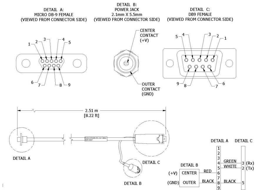
Figure 41 -RS232 Communications and power cable
