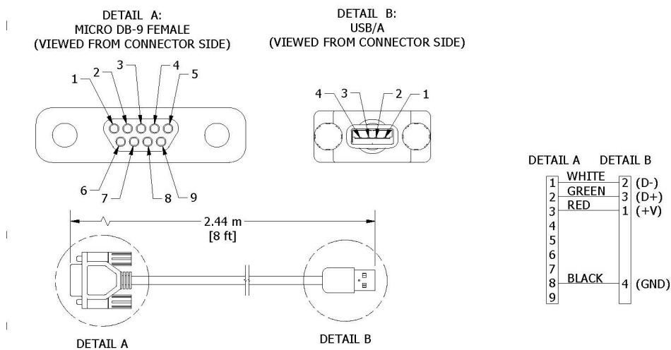
Figure 42 -USB Communications cable
