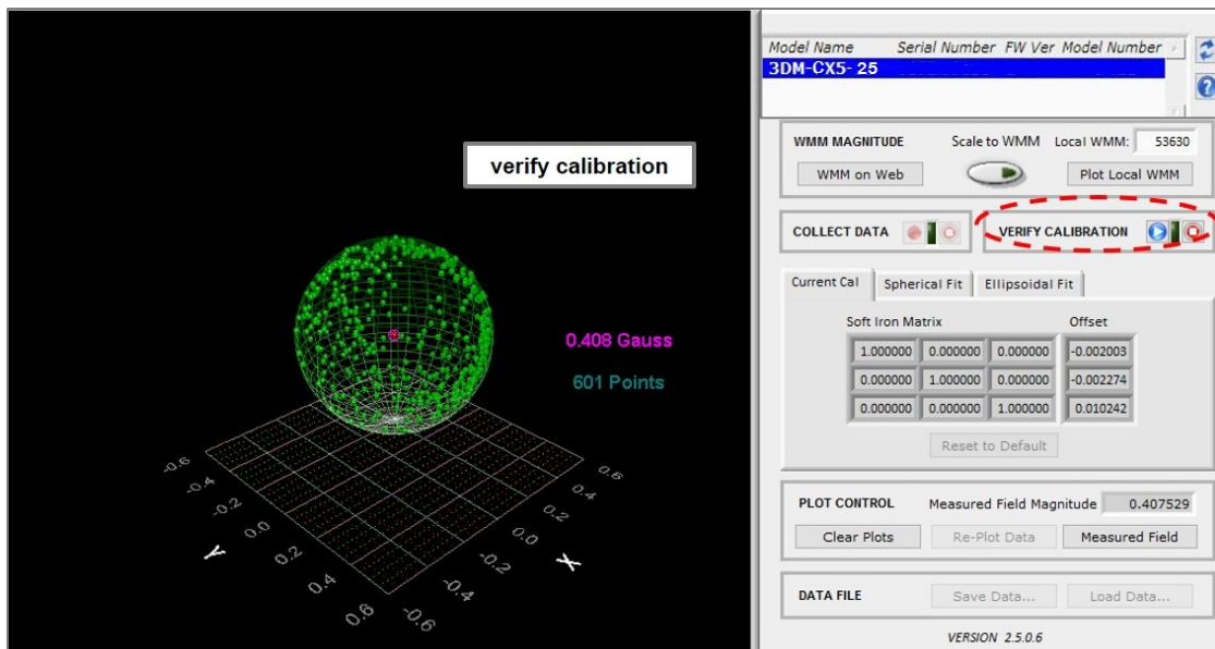
Figure 28 -Verify Calibration
