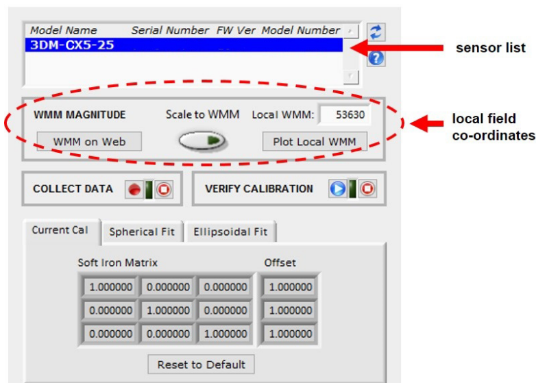
Figure 26 -Sensor Menu
