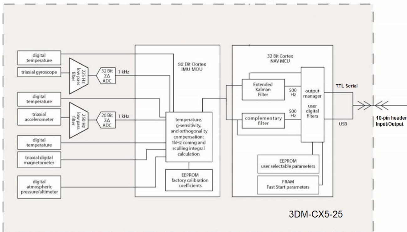
Figure 14 -3DM-CX5-25 Block Diagram
