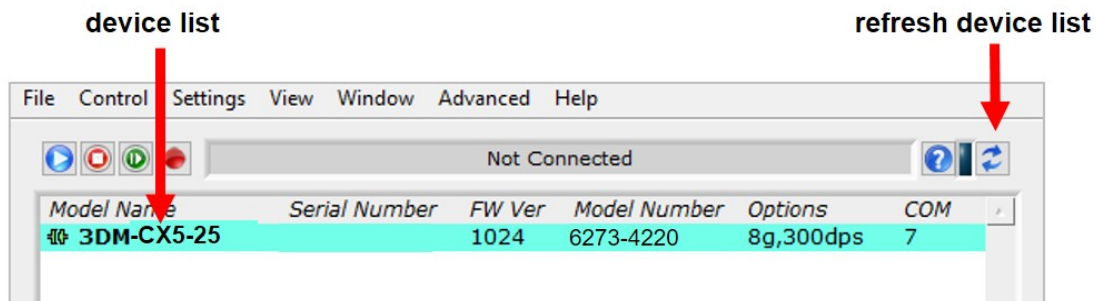
Figure 7 -Sensor Communication
