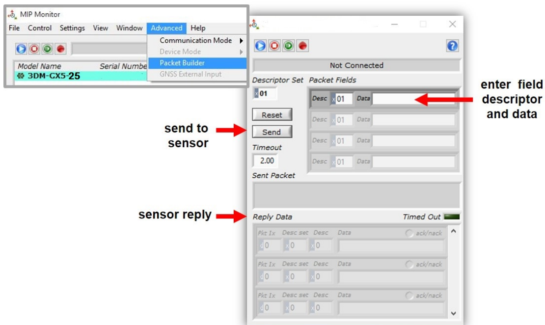
Figure 35 -Packet Builder
