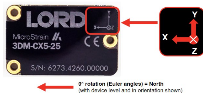
Figure 19 -Sensor Frame
