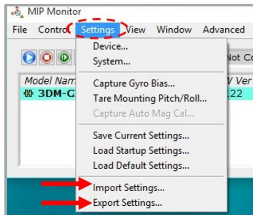
Figure 33 -Import/Export Settings Menu
