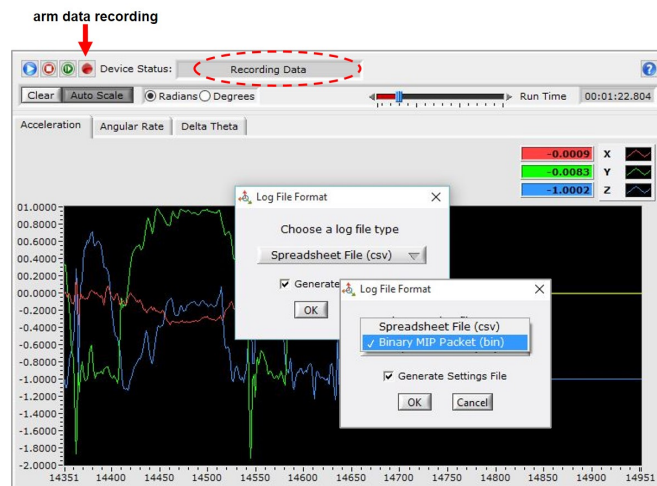
Figure 12 -Data Recording
