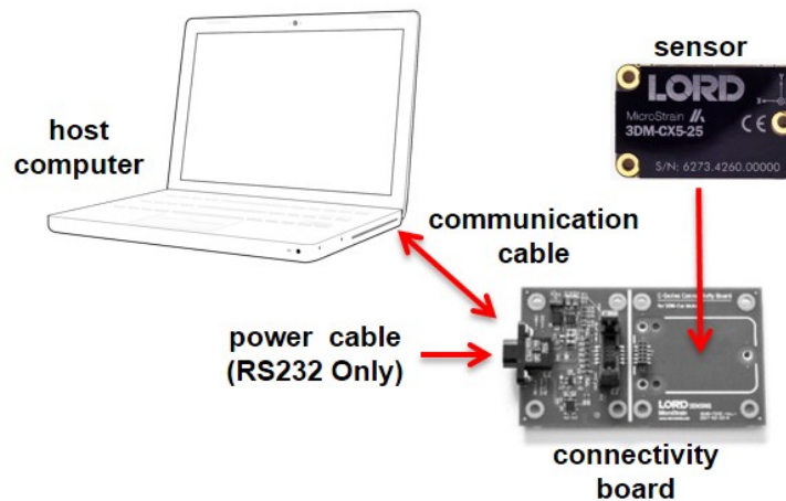
Figure 4 -System Connections
