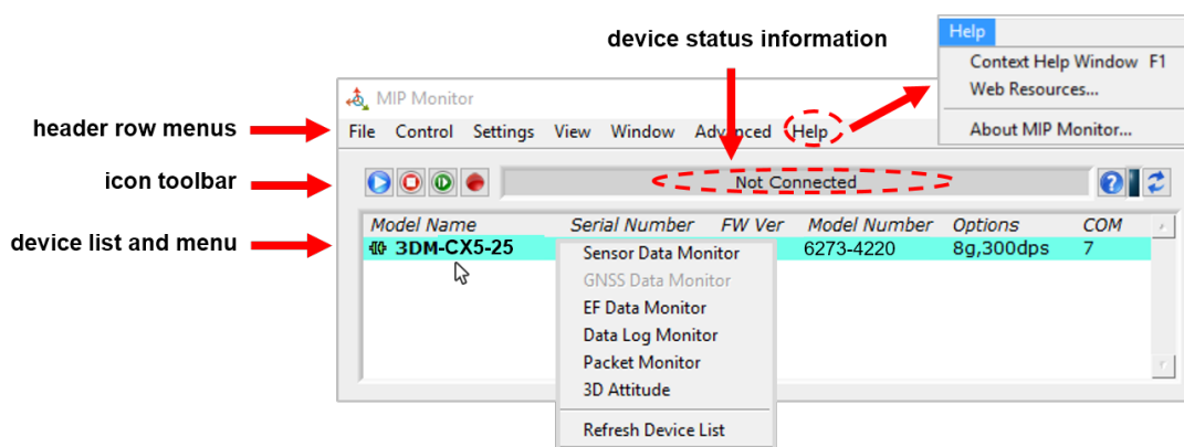
Figure 5 - Main Window Display
