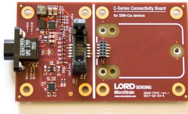
Figure 39 -C-Series Connectivity Board
