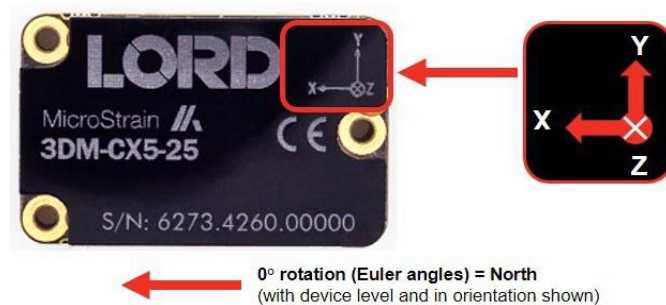
Figure 19 -Sensor Frame
