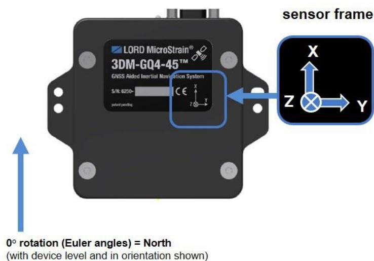
Figure 21 - Sensor Frame
