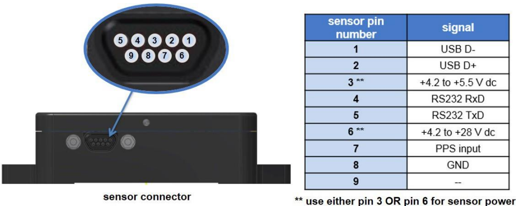
Figure 36 - Connector Wiring
