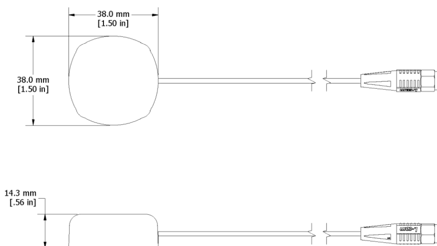
Figure 32 - GNSS Antenna
