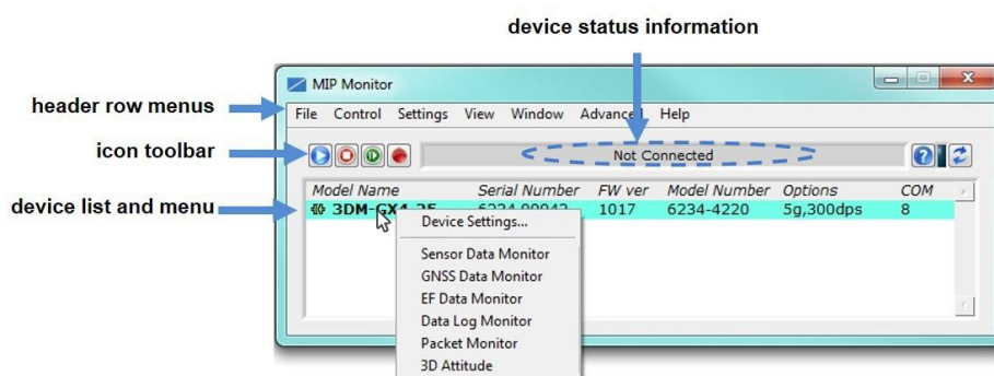
Figure 6 - Main Window
