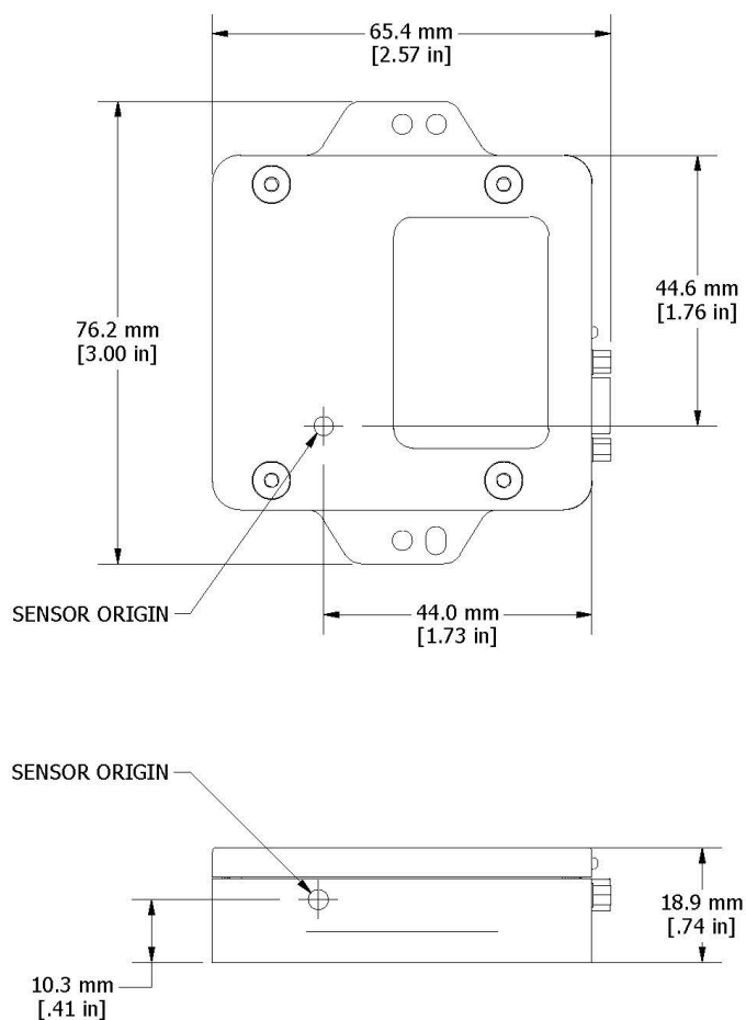
Figure 41 - 3DM-GQ4™ Sensor Origin
