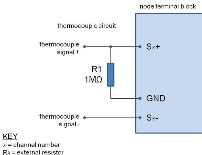
Figure 38 - Connecting a Thermocouple
