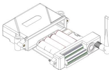
Figure 60 - Replace Batteries
