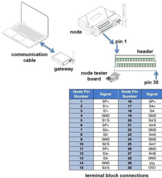
Figure 6 - System Connections
