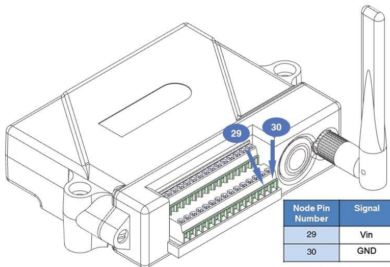
Figure 53 - External Power Connection
