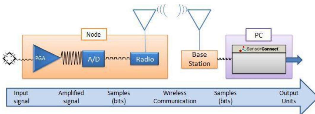
Figure 32 - Differential Channel Signal Processing
