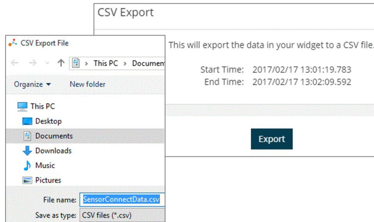
Figure 31. Exporting Data
