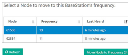
Figure 7. Move Node
