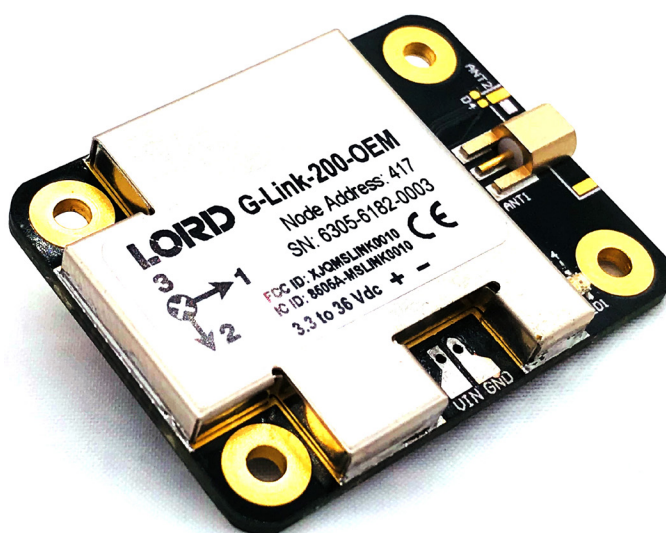
Figure 1. G-Link-200-OEM
