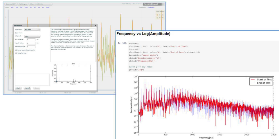
Figure 26. MathEngine® View
