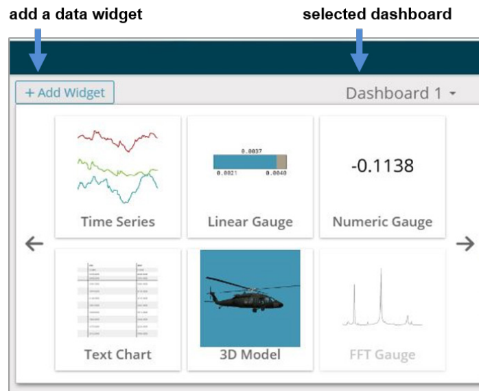
Figure 28. Viewing Data
