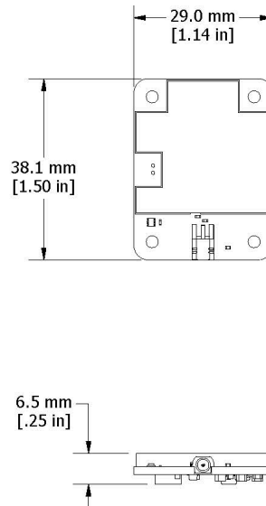
Figure 32. Mounting the Node
