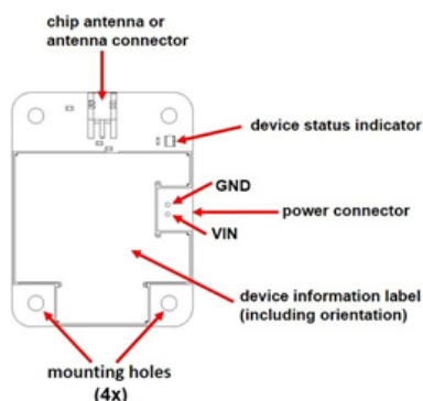
Figure 2. Interface and Indicators
