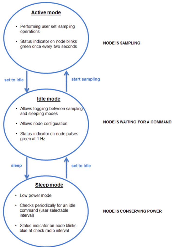
Figure 3. Node Operational Modes
