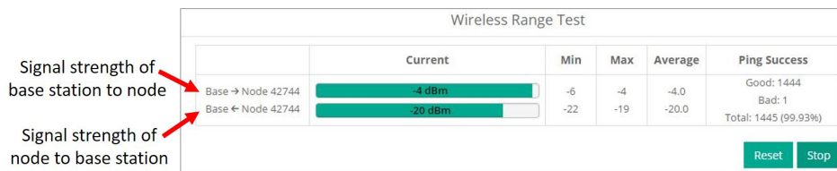
Figure 35. Range Test Statistics
