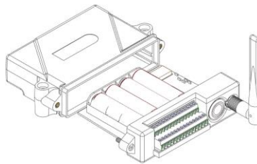
Figure 60 - Replace Batteries
